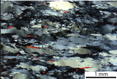
Sample 33, Hendry's Creek, 10.2% mica
